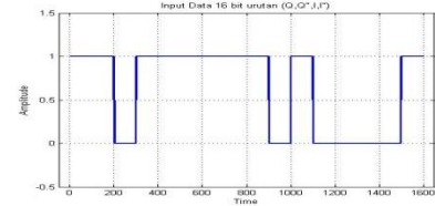
Gambar 7. Sinyal Digital 16-QAM
