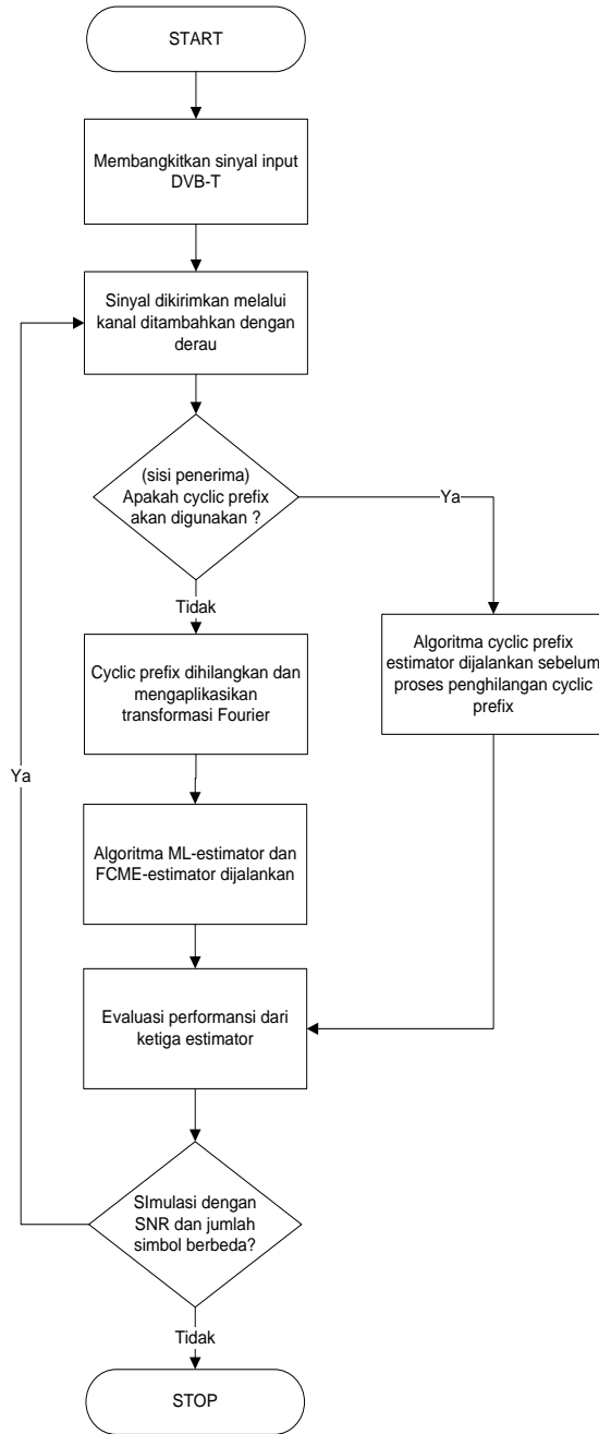
Gambar 1. Flowchart Simulasi
