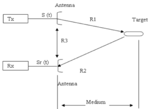
Gambar 1. Blok diagram radar Sederhana
