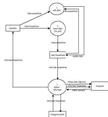
Gambar 10.DFD Level 1
