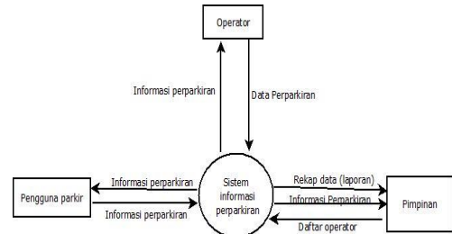
Gambar 9. DFD Level 0
