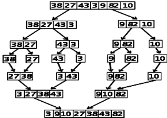
Gambar 5. Ilustrasi Merge Sort
