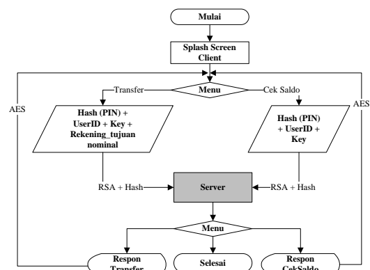
Gambar 2. Flowchart Client
