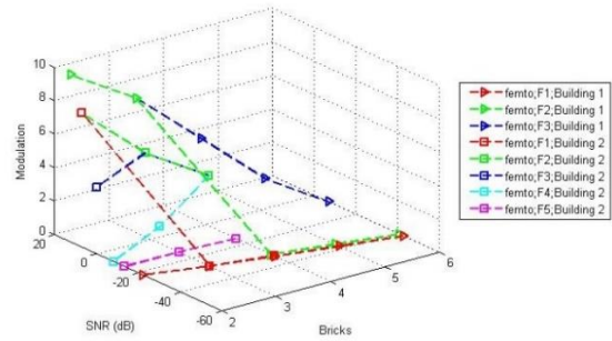
Fig. 6. AMC Modulation Femtocell at The Building
