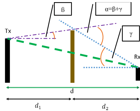
Fig. 2. Single Knife-Edge Diffraction Model
