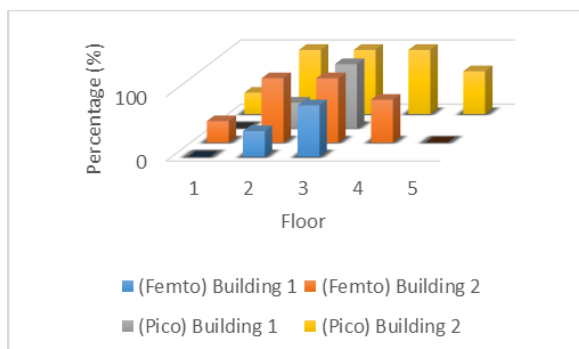
Fig. 9. The Percentage Coverage Area for Femtocell and Picocell
