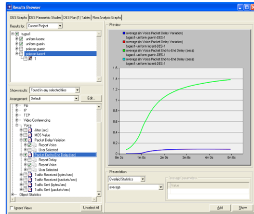
Gambar 10 End To End Delay Voice Guerin dan Lucent (Uniform QoS Default)
