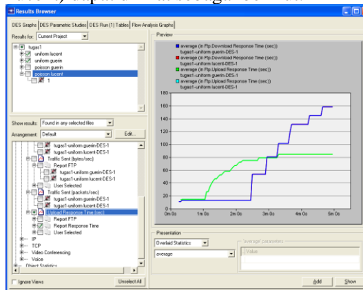
Gambar 8 Response Download dan Upload FTP Guerin dan Lucent (Uniform QoS Default)
