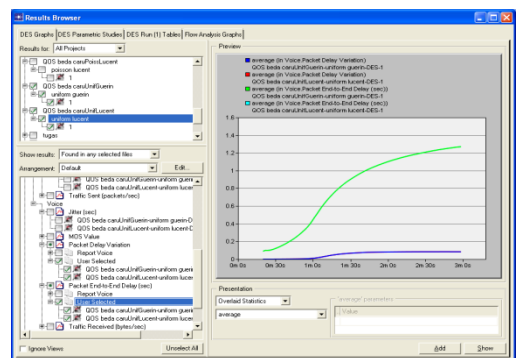
Gambar 16 End To End Delay Voice Guerin dan Lucent (Uniform Qos Beda)
