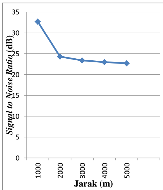
Gambar 3 Grafik jarak terhadap SNR ( Signal to Noise Ratio )
